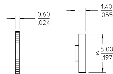
INSULATOR
