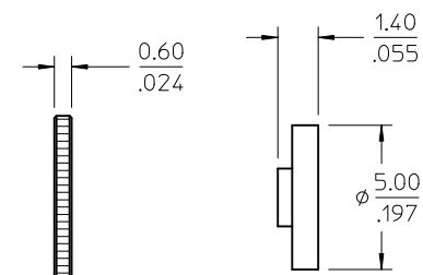
INSULATOR
