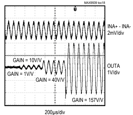
GAIN ADJUST RESPONSE
