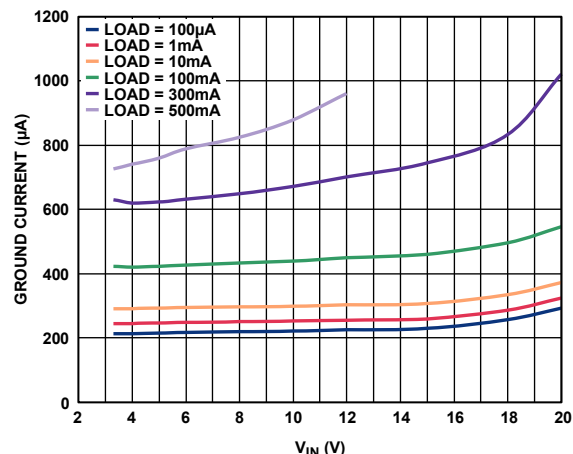
Figure 28. Ground Current vs. Input Voltage, V_{OUT} = 1.8 V
