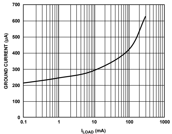
Figure 27. Ground Current vs. Load Current, V_{OUT} = 1.8 V
