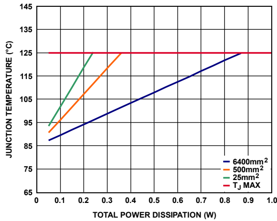
Figure 75. SOIC, T A = 85°C
