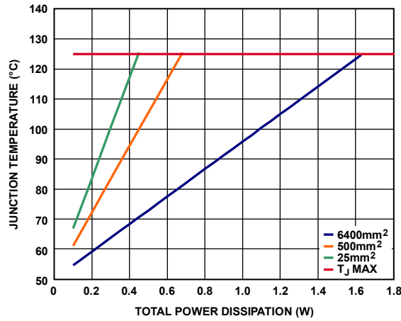
Figure 74. SOIC, T A = 50°C
