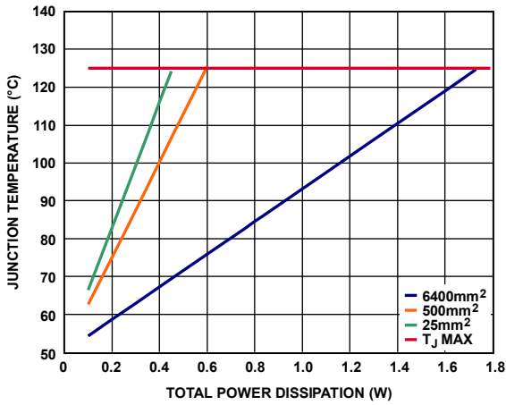
Figure 71. LFCSP, T A = 50°C
