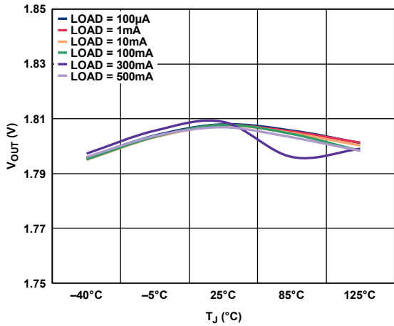
Figure 23. Output Voltage vs. Junction Temperature, V_{OUT} = 1.8 V
