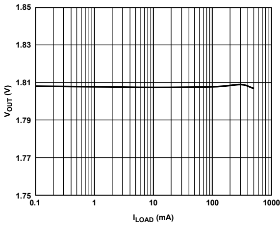
Figure 24. Output Voltage vs. Load Current, V_{OUT} = 1.8 V
