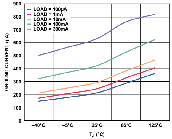
Figure 26. Ground Current vs. Junction Temperature, V_{OUT} = 1.8 V
