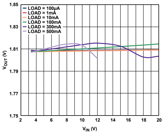
Figure 25. Output Voltage vs. Input Voltage, V_{OUT} = 1.8 V
