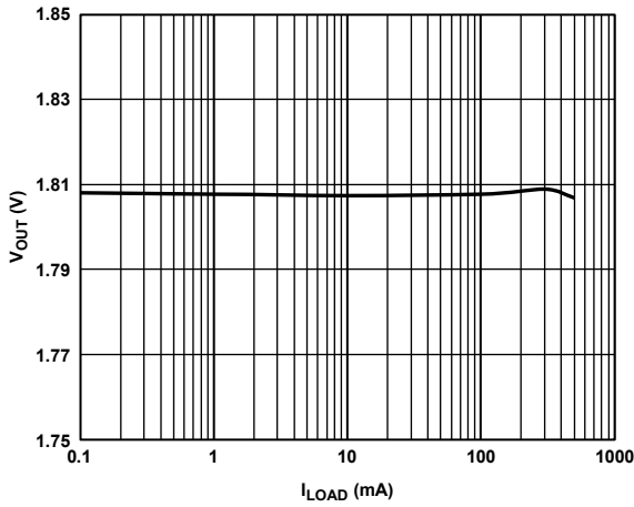
Figure 24. Output Voltage vs. Load Current, V_{OUT} = 1.8\text{ V}
