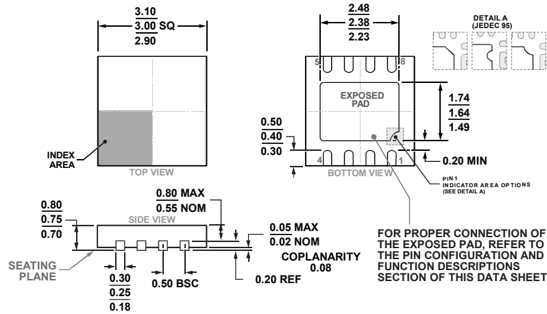
COMPLIANT TO JEDEC STANDARDS MO-229-WEED-4 Figure 80. 8-Lead Lead Frame Chip Scale Package [LFCSP_WD] 3 mm × 3 mm Body, Very Thin, Dual Lead (CP-8-5) Dimensions shown in millimeters
