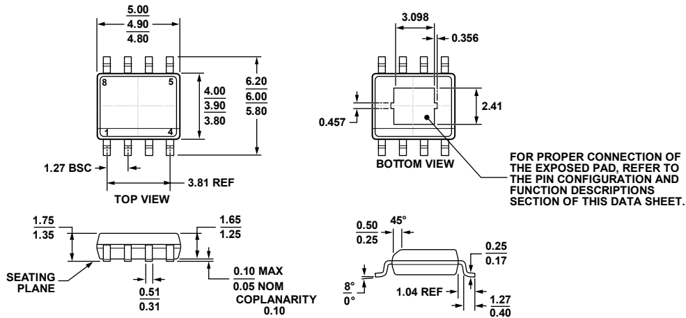
COMPLIANT TO JEDEC STANDARDS MS-012-AA Figure 81. 8-Lead Standard Small Outline Package, with Exposed Pad [SOIC_N_EP] Narrow Body (RD-8-2) Dimensions shown in millimeters
