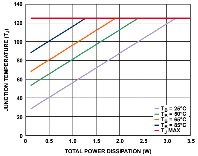
Figure 77. SOIC
