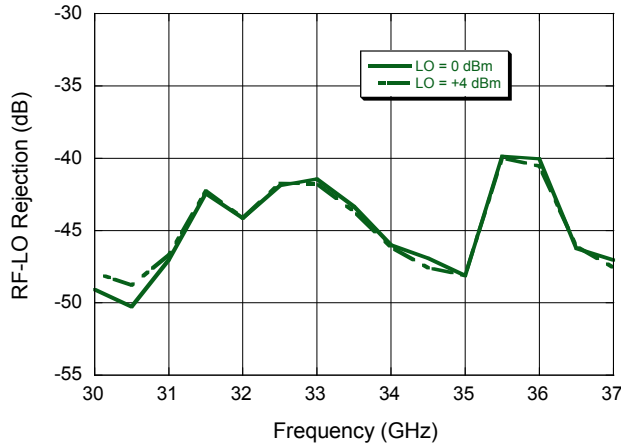
RF-LO Rejection
