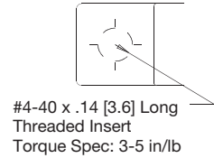
Threaded Mounting Flange 46XX-XXX5 Detail A
