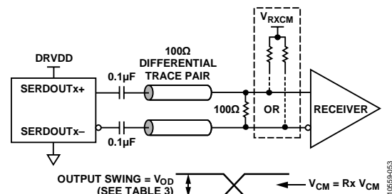
Figure 57. AC-Coupled Digital Output Termination Example
