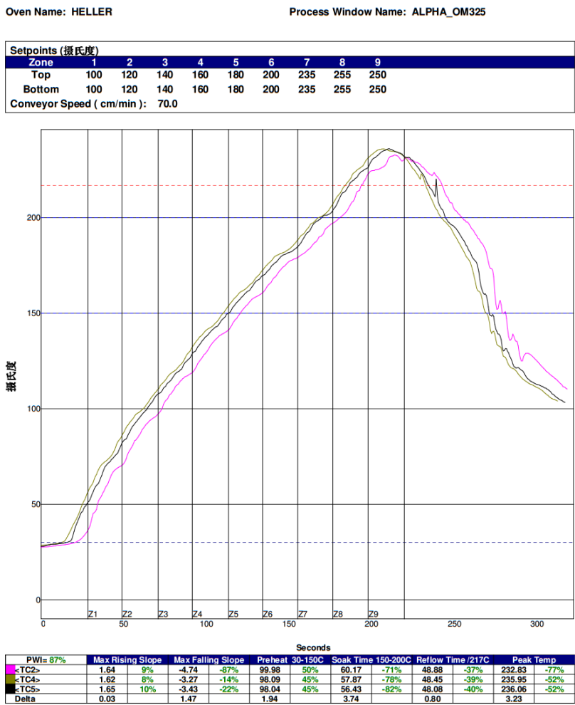
Figure 6 - Example solder reflow profile (AMWx36-E03 evaluation board)
