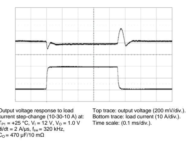
Output Load Transient Response, Default PID/NLR
