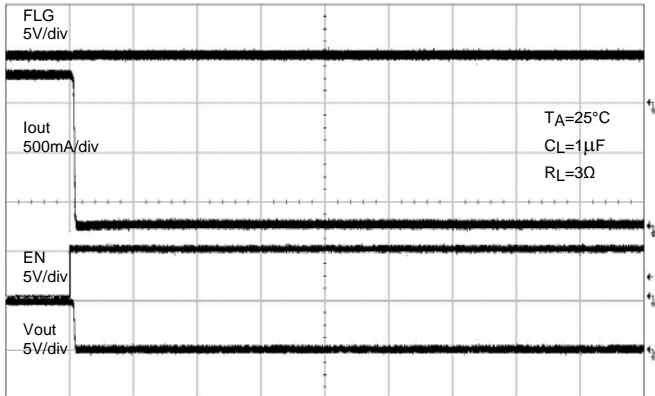
Device Disabled
