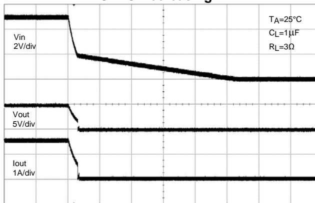
UVLO Decreasing
