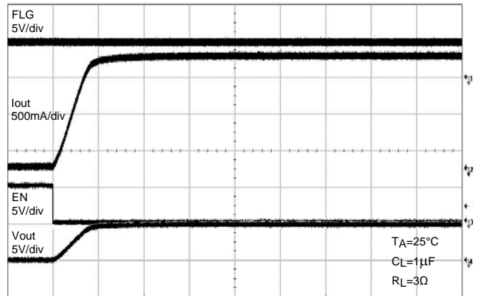
Device Enabled
