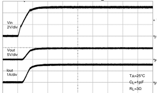
UVLO Increasing
