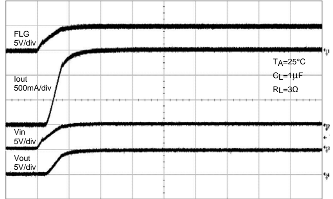
Power On
