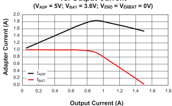
Adapter Charging Current vs. Output Current
