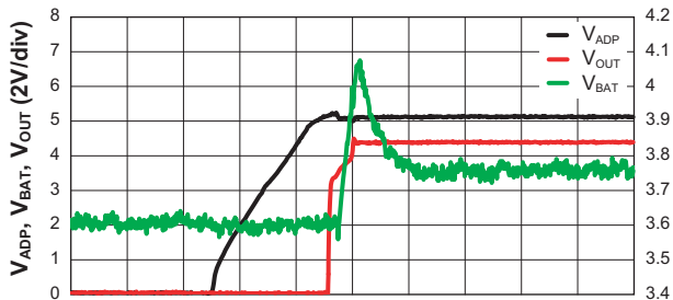
Response of Out when Switching from V_{BAT} to V_{ADP}
