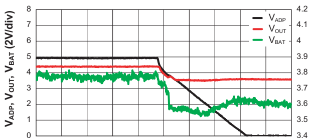
Response of Out when Switching from V_{ADP} to V_{BAT}
