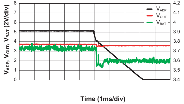
Response of Out when \overline{EN}_O = 5V ( V_{ADP} = 5V \rightarrow 0V ; V_{BAT} = 3.6V ; R_{LOAD} = 50\Omega ; \overline{EN}_{BAT} = 0V ; C_{OUT} = 10\mu F )
