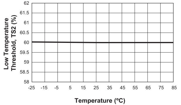
Low Temperature Threshold ( V_{ADP} = 5V )
