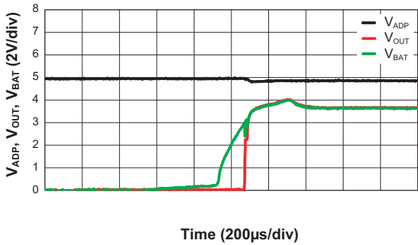
Response of Out when Inserting Battery ( V_{BAT} = 0V \rightarrow 3.6V ; V_{ADP} = 5V ; R_{LOAD} = 50\Omega ; \overline{EN}_{BAT} = 0V ; \overline{EN}_O = 0V ; C_{OUT} = 10\mu F )
