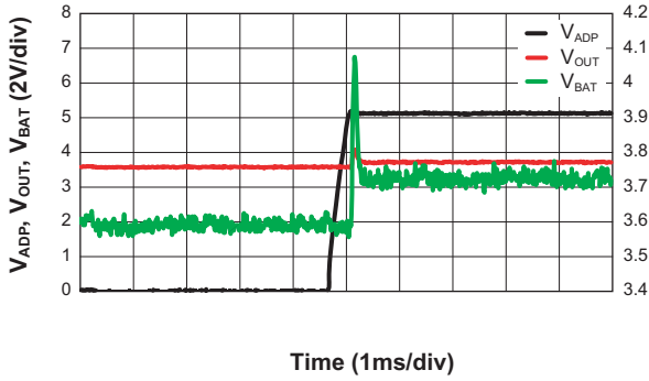
Response of Out when \overline{EN}_O = 5V ( V_{ADP} = 0V \rightarrow 5V ; V_{BAT} = 3.6V ; R_{LOAD} = 50\Omega ; \overline{EN}_{BAT} = 0V ; C_{OUT} = 10\mu F )
