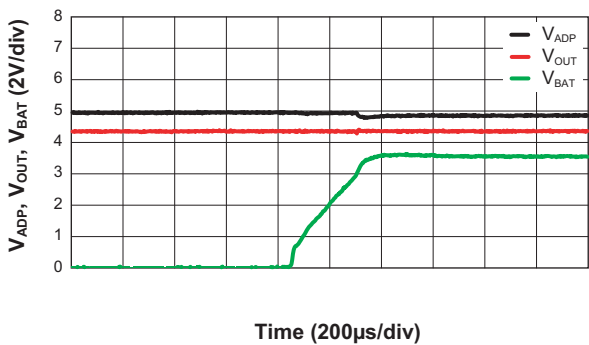
Response of Out when Inserting Battery ( V_{BAT} = 0V \rightarrow 3.6V ; R_{LOAD} = 50\Omega ; V_{ADP} = 5V ; \overline{EN}_{BAT} = 5V ; \overline{EN}_O = 0V ; C_{OUT} = 10\mu F )
