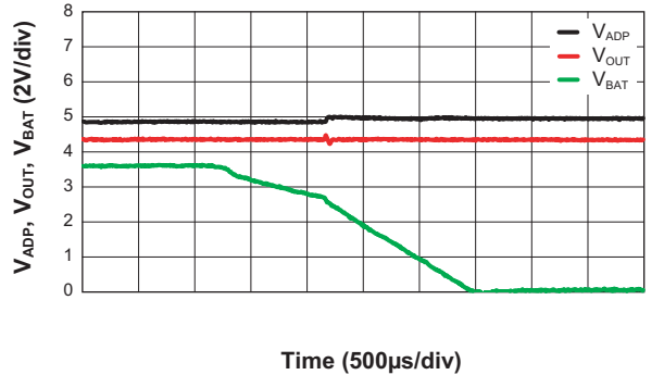
Response of Out when Removing Battery ( V_{BAT} = 4.1V \rightarrow 0V ; V_{ADP} = 5V ; R_{LOAD} = 50\Omega ; \overline{EN}_{BAT} = 5V ; \overline{EN}_O = 0V ; C_{OUT} = 10\mu F )
