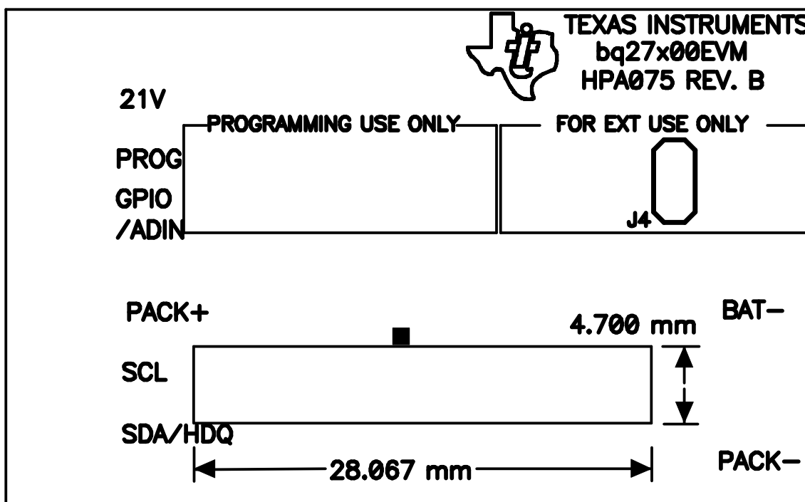
Figure 3. bq27200EVM Silkscreen
