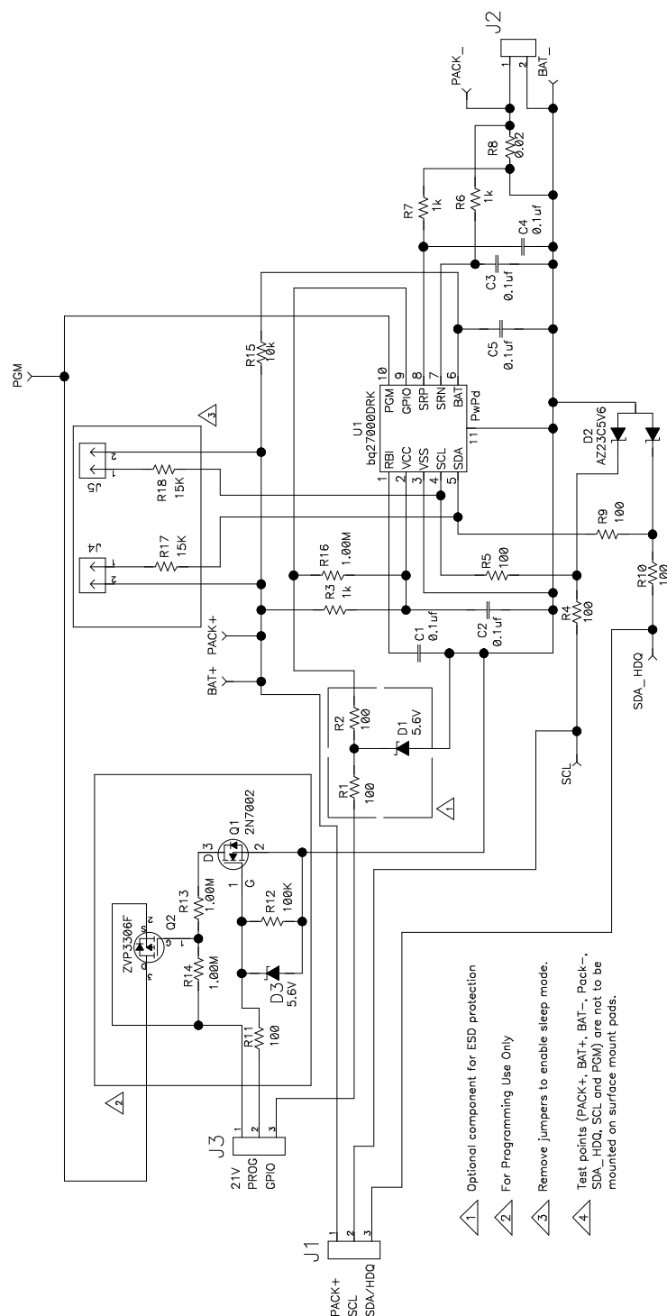
Figure 1. bq27200EVM Schematic
