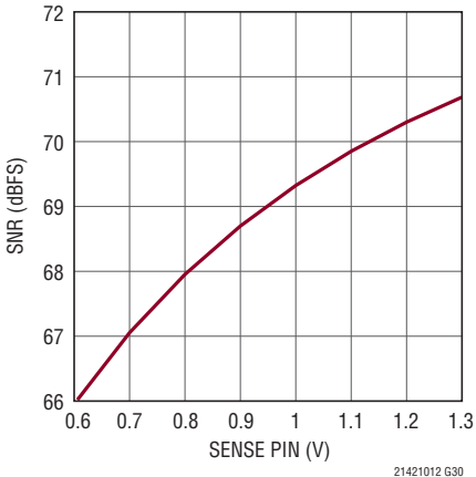
LTC2141-12: SNR vs SENSE, f_{IN} = 5\text{MHz} , -1dBFS
