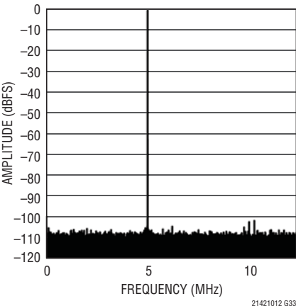
LTC2140-12: 64k Point FFT, f_{IN} = 5\text{MHz} , -1dBFS, 25MSPS
