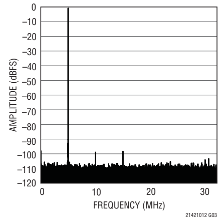
LTC2142-12: 64k Point FFT, f_{IN} = 5\text{MHz} , -1\text{dBFS} , 65Mps
