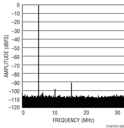
LTC2142-12: 64k Point FFT, f_{IN} = 70\text{MHz} , -1\text{dBFS} , 65Mps
