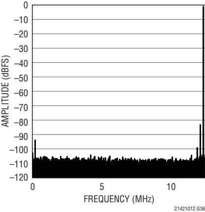
LTC2140-12: 64k Point FFT, f_{IN} = 140\text{MHz} , -1dBFS, 25MSPS
