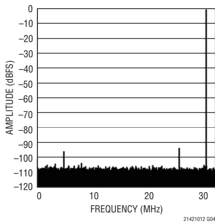
LTC2142-12: 64k Point 2-Tone FFT, f_{IN} = 69\text{MHz} , 70\text{MHz} , -7\text{dBFS} , 65Mps
