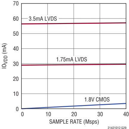
LTC2141-12: I_{O_VDD} vs Sample Rate, 5MHz, -1dBFS, Sine Wave Input on Each Channel
