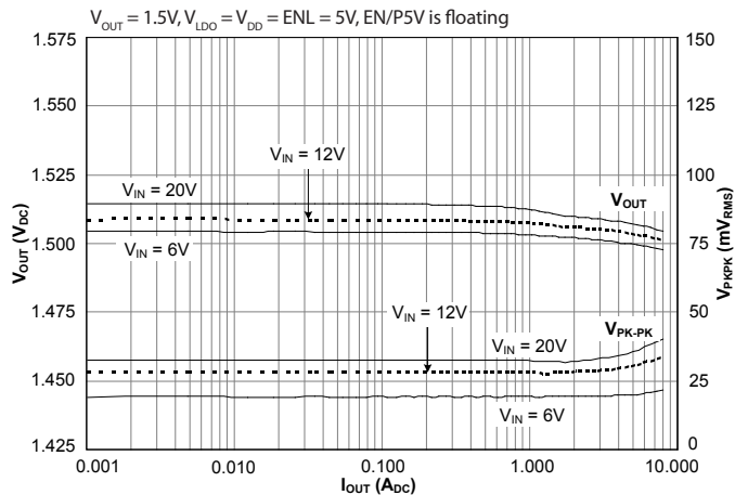
V_{OUT} vs. Load — Forced Continuous Mode
