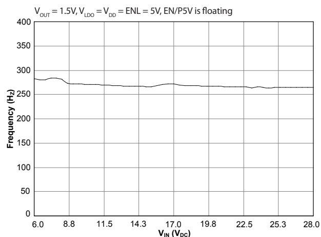
Frequency vs. Line — FCM Mode
