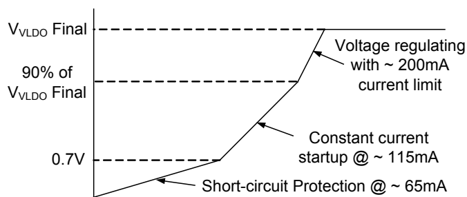
Figure 11 — LDO Start-Up
