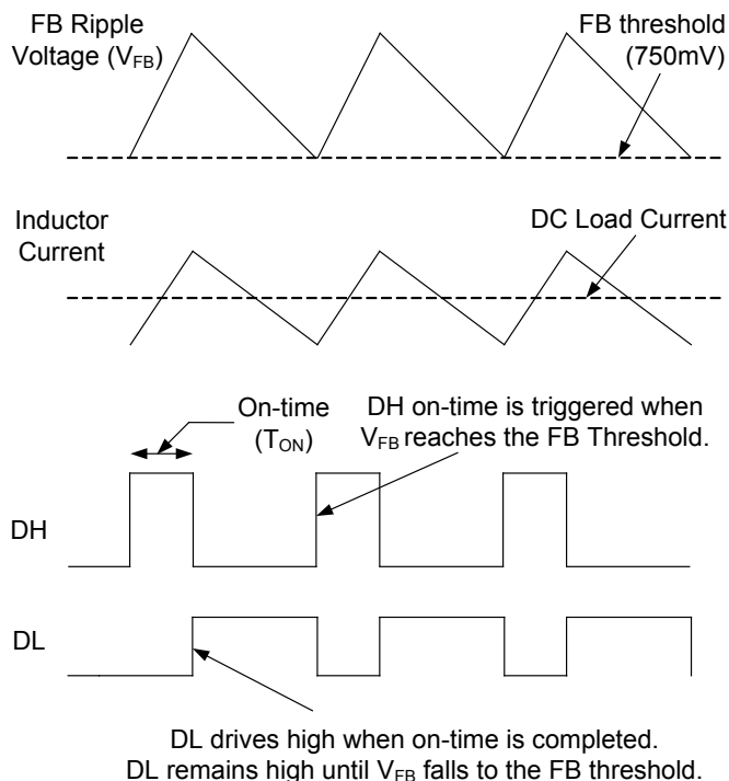
Figure 4 — Forced Continuous Mode Operation
