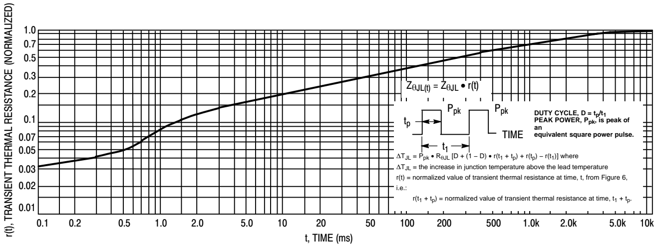
Figure 6. Thermal Response
