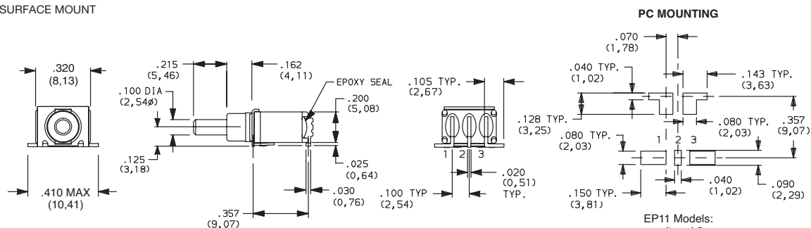
EP12SD1SAPE SPDT
