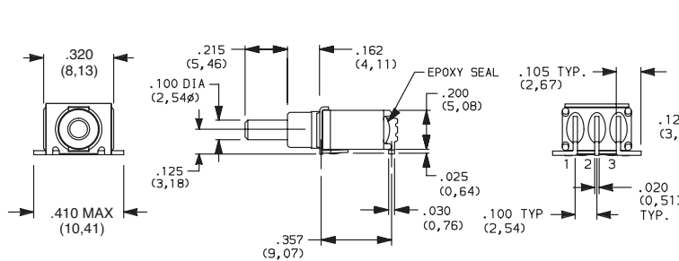
EP12SD1SAPE SPDT
