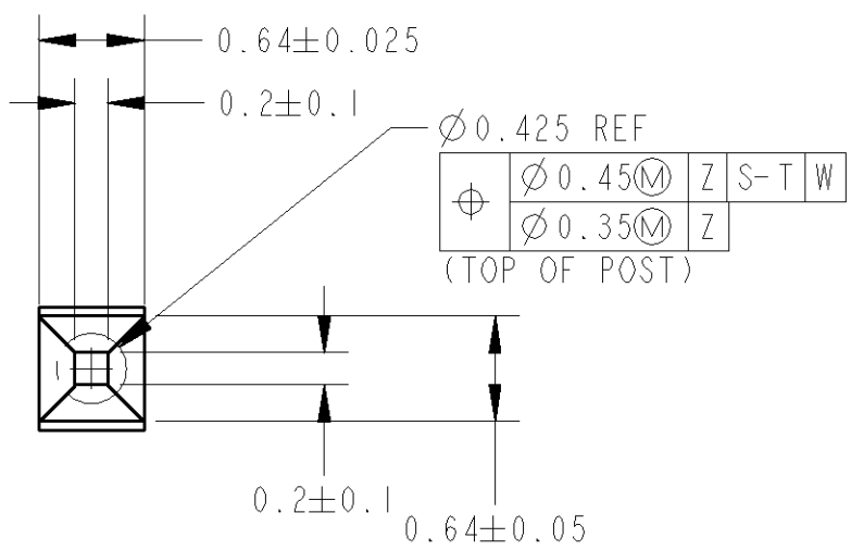
DETAIL C SCALE 20:1
