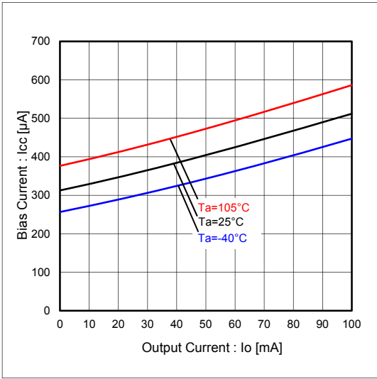
Figure 19. I_O - I_{CC}
