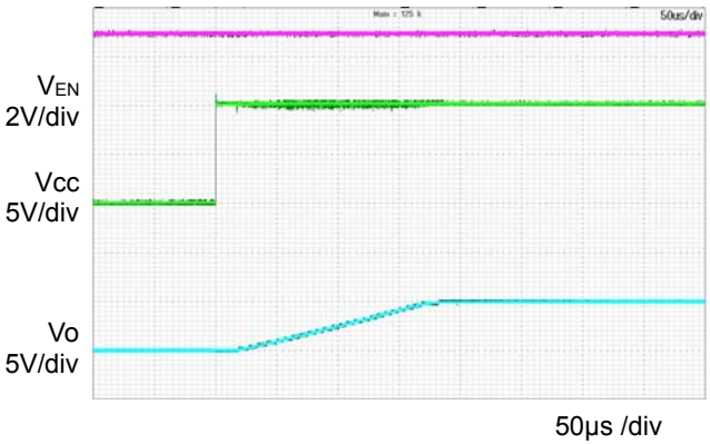
Figure 3. Input sequence (Ta=-40°C) (VCC = 0V→10V)
