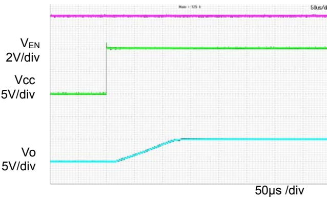
Figure 4. Input sequence (Ta=105°C) (VCC = 0V→10V)
