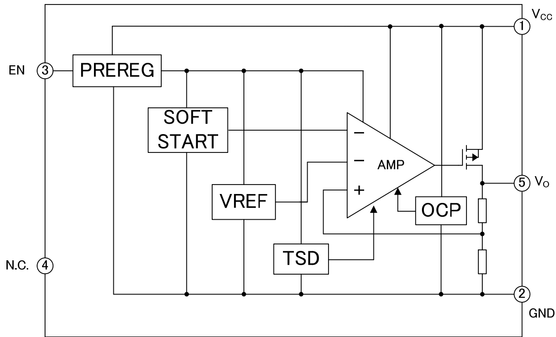
Figure 1. Block Diagram
