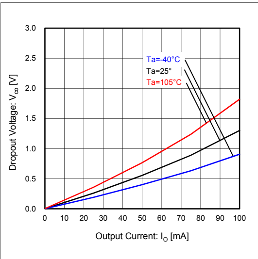
Figure 21. Minimum Dropout Voltage ( V_{CC}=4.75\text{V} )
