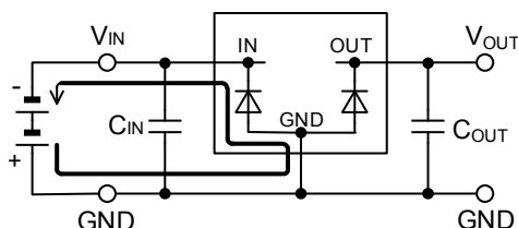
Figure 30. Current Path in Reverse Input Connection
