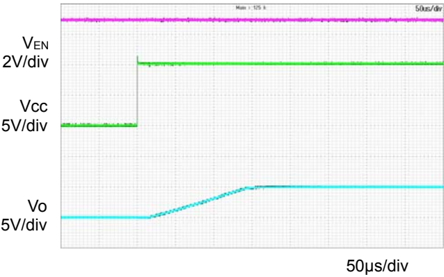
Figure 2. Input sequence (Ta=25°C) (VCC = 0V→10V)
