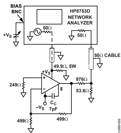
Figure 56. Positive PSRR
