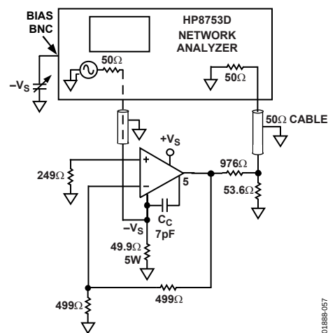
Figure 57. Negative PSRR
