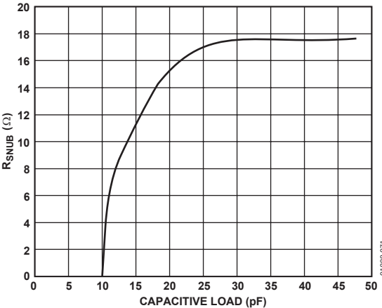
Figure 71. Relationship of R_{\text{SNUB}} vs. C_L for 2 dB Peaking at a Gain of +2
