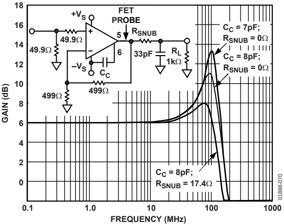
Figure 70. Peaking vs. R_{\text{SNUB}} and C_C for C_L = 33\text{pF}
