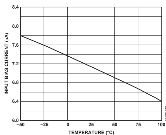
Figure 40. Input Bias Current vs. Temperature
