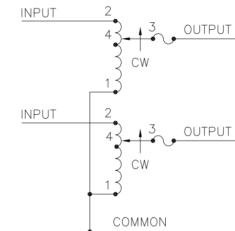
SCHMATIC FUSE RECOMMENDED BUT NOT SUPPLIED
