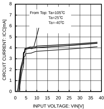
Fig.7 Circuit Current (BD9006F/HFP, BD9007F/HFP)
