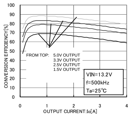
Fig.25 Efficiency f=500kHz (BD9009HFP)
