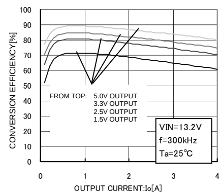
Fig.24 Efficiency f=300kHz (BD9009HFP)
