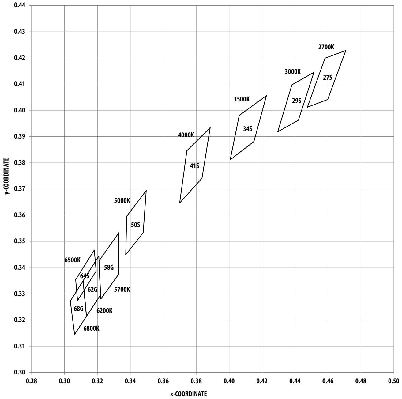
Figure 2 Chromaticity Diagram
