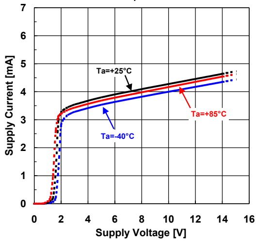
Supply Current vs. Supply Voltage G_V=0\text{dB}
