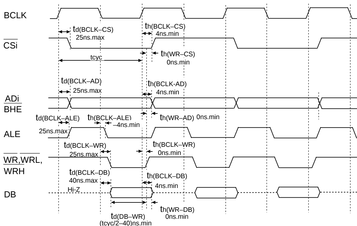
Figure 1.23.4. V_{CC} = 5V timing diagram (3)
