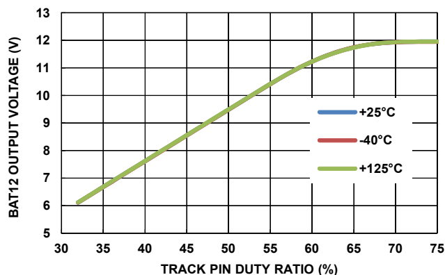
FIGURE 22. BAT12 OUTPUT VOLTAGE (DIGITAL TRACKING MODE, FTRK = 500kHz, BUCK MODE, DE MODE, PHASE DROP DISABLED, f_{CLK} = 100kHz )
