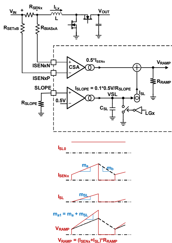
FIGURE 136. SLOPE COMPENSATION BLOCK DIAGRAM
