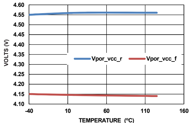
FIGURE 119. V CC POWER-ON RESET VOLTAGE, RISING AND FALLING
