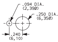
With Standard Locking Ring
