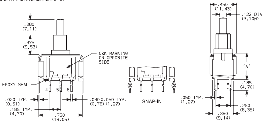
8261SH9_BE2 DPDT
