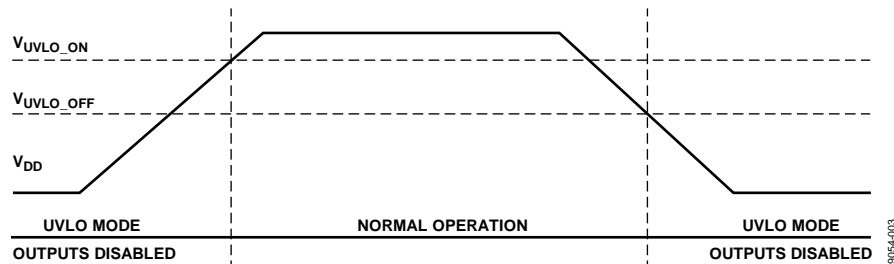
Figure 3. UVLO Function
