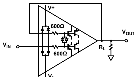
Figure 50. Input ESD Diode Current Limiting, Unity Gain
