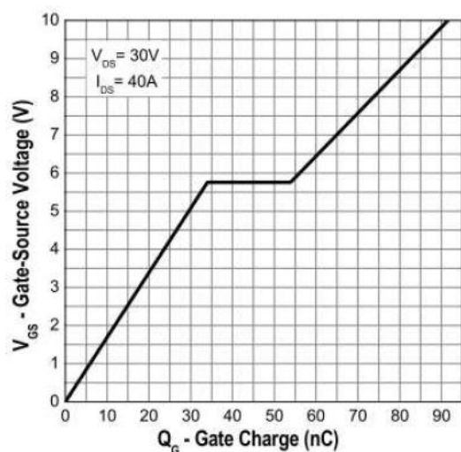
Gate Charge
