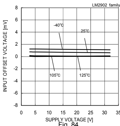
Fig. 84 Input Offset Voltage – Supply Voltage ( V_{icm}=0[V] , V_{OUT}=1.4[V] )
