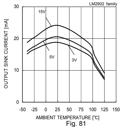
Fig. 81 Output Sink Current – Ambient Temperature ( V_{OUT}=V_{CC} )
