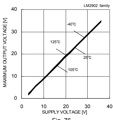
Fig. 76 Maximum Output Voltage – Supply Voltage ( R_L=10[k\Omega] )
