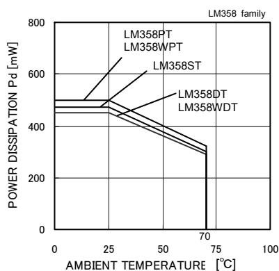
Fig. 1 Derating Curve
