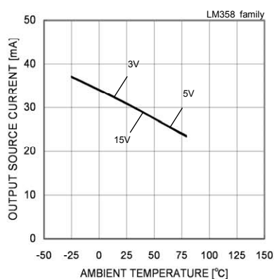
Fig. 7 Output Source Current – Ambient Temperature ( V_{OUT}=0[V] )
