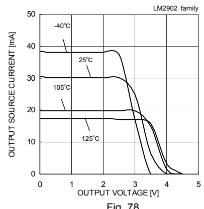
Fig. 78 Output Source Current – Output Voltage ( V_{CC}=5[V] )
