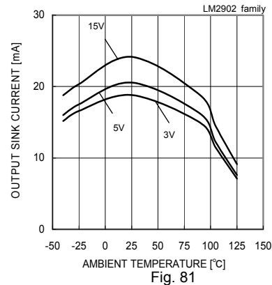
Fig. 81 Output Sink Current – Ambient Temperature ( V_{OUT}=V_{CC} )
