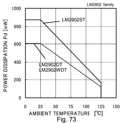
Fig. 73 Derating Curve
