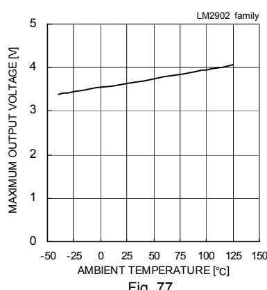
Fig. 77 Maximum Output Voltage – Ambient Temperature ( V_{CC}=5[V] , R_L=2[k\Omega] )
