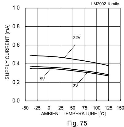
Fig. 75 Supply Current – Ambient Temperature
