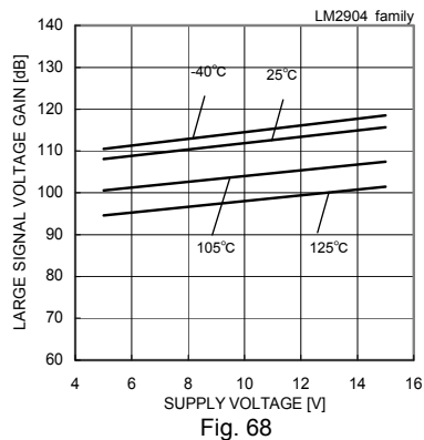
Fig. 68 Large Signal Voltage Gain – Supply Voltage ( R_L=2[k\Omega] )
