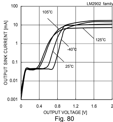
Fig. 80 Output Sink Current – Output Voltage ( V_{CC}=5[V] )
