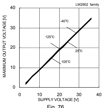
Fig. 76 Maximum Output Voltage – Supply Voltage ( R_L=10[k\Omega] )
