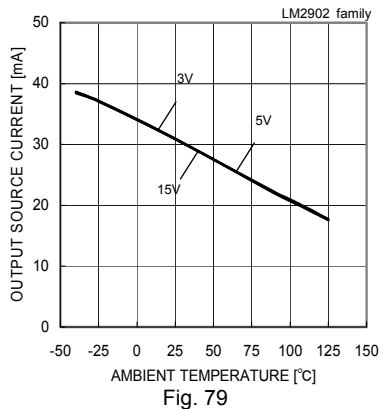
Fig. 79 Output Source Current – Ambient Temperature ( V_{OUT}=0[V] )
