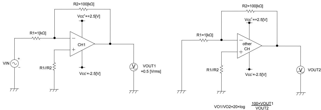
Fig.101 Measurement Circuit3
