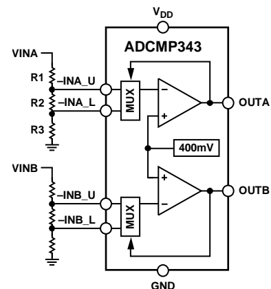
Figure 2. ADCMP343
