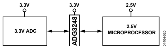
Figure 20. Level Translation Between a 3.3 V ADC and a 2.5 V Microprocessor
