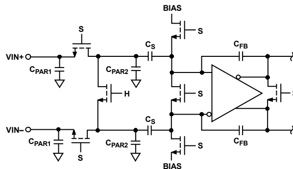
Figure 46. Switched-Capacitor Input
