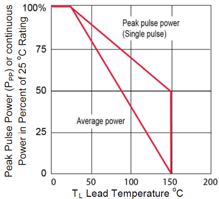
Figure 3 • Derating Curve
