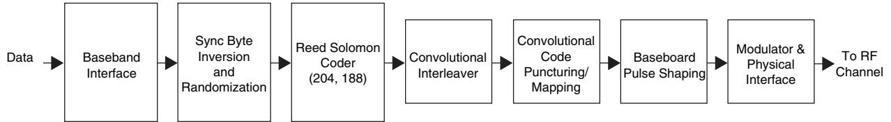
Figure 2-3. Broadband Wireless Access System
