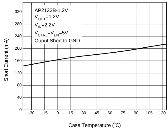
Figure 13. Short Current vs. Case Temperature
