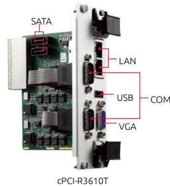
cPCI-R3610T
