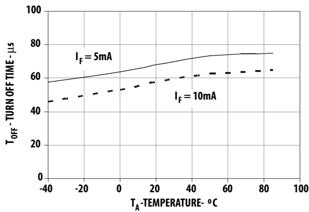
Figure 15. Typical Turn Off Time vs Temperature
