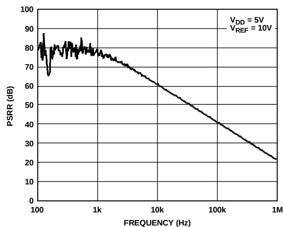
Figure 17. AD5544/AD5554 Power Supply Rejection vs. Frequency
