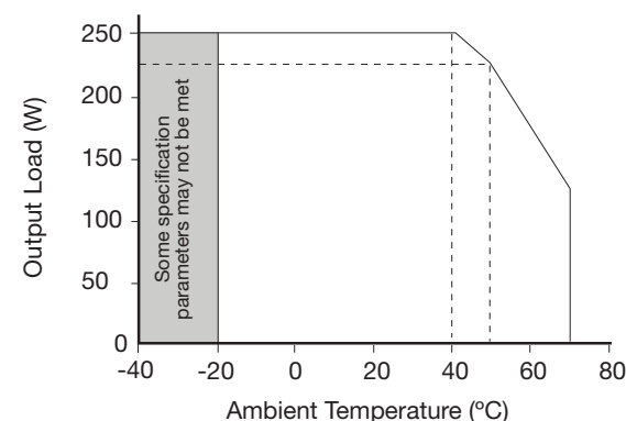
Figure 9 - Convection-cooled
